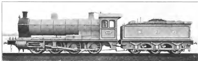
Fig. 5032. Eight-Coupled Goods Locomotive. North Eastern Railway. Cylinders 20 in. x 26 in.; Total Heating Surface 1,675 sq. ft.; Diameter of Drivers 55¾ in.; Weight on Drivers 140,600 lbs.; Total Weight 140,600 lbs.
